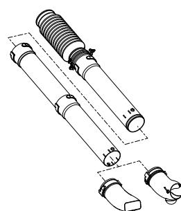
0G.345.00 KIT FOR BLOWING
