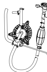
0G.340.00 BOOSTER AND FILLING PUMP
